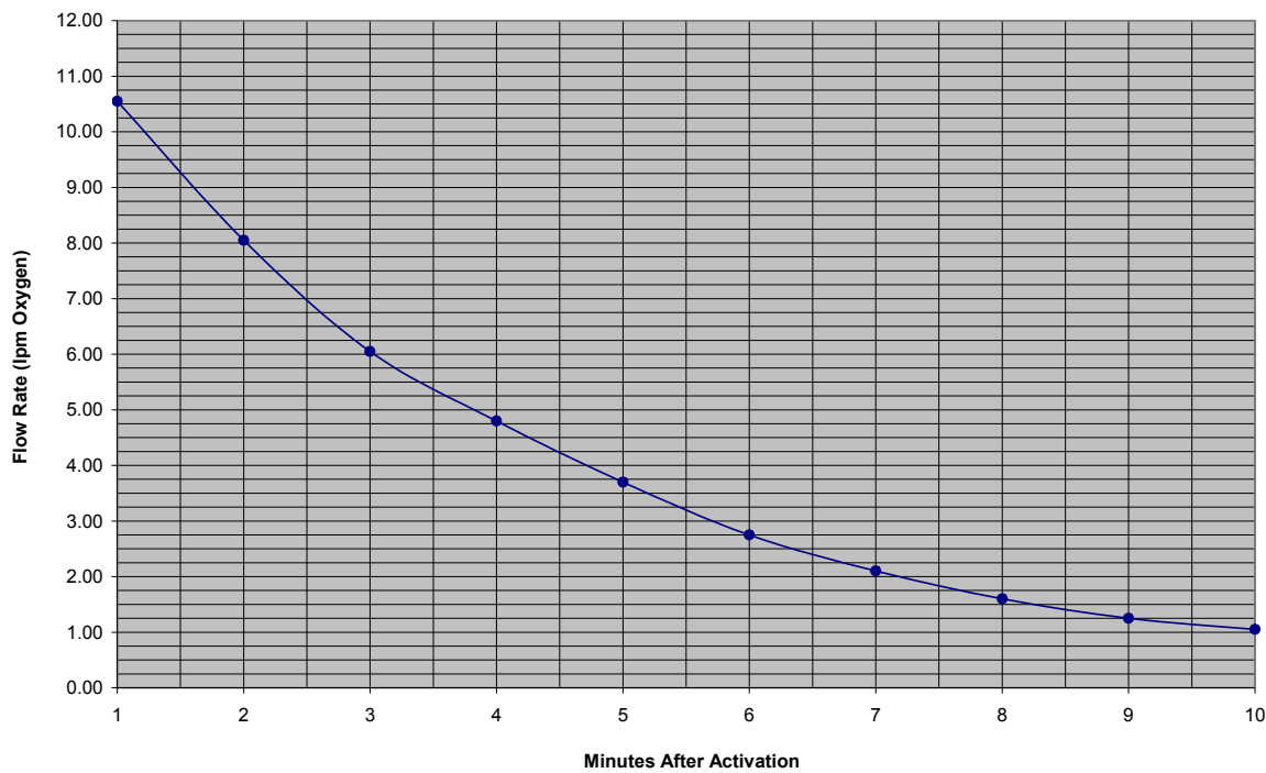
Flow Characteristics of "Single Bottle" Bailout Systems
